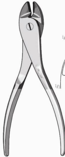
SIDE BITE WIRE CUTTER 22-523-18 7" (178mm) welded carbide jaws cuts up to .062" (1.6mm)
