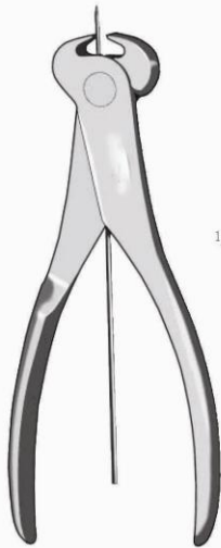
CANNULATED PIN CUTTER 22-520-18 7 1/2" (191mm) cuts up to .062" (1.6mm)
