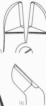
SIDE BITE WIRE CUTTER 22-523-18 7" (178mm) welded carbide jaws cuts up to .062" (1.6mm)
